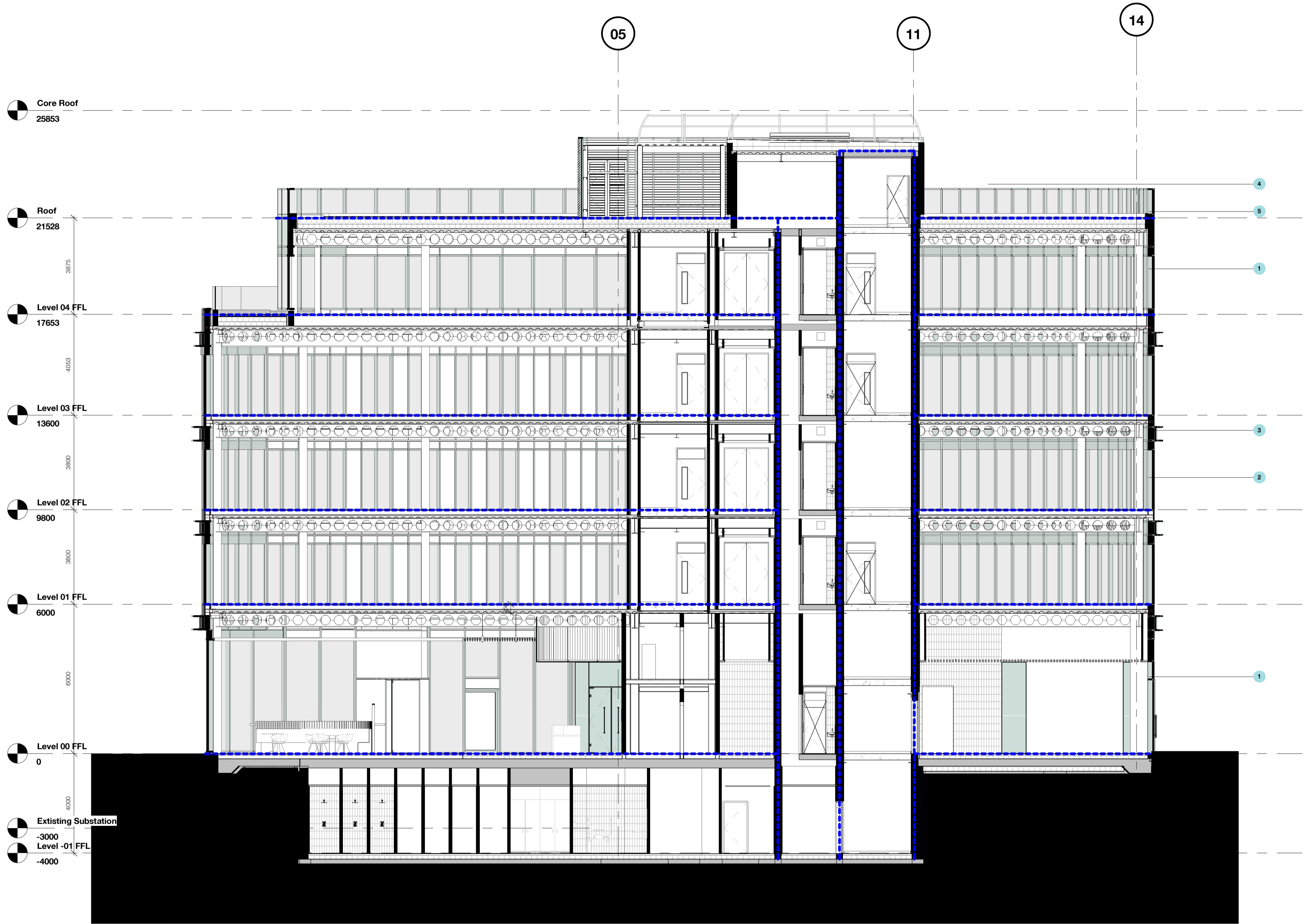
1 Section 1 1:100
