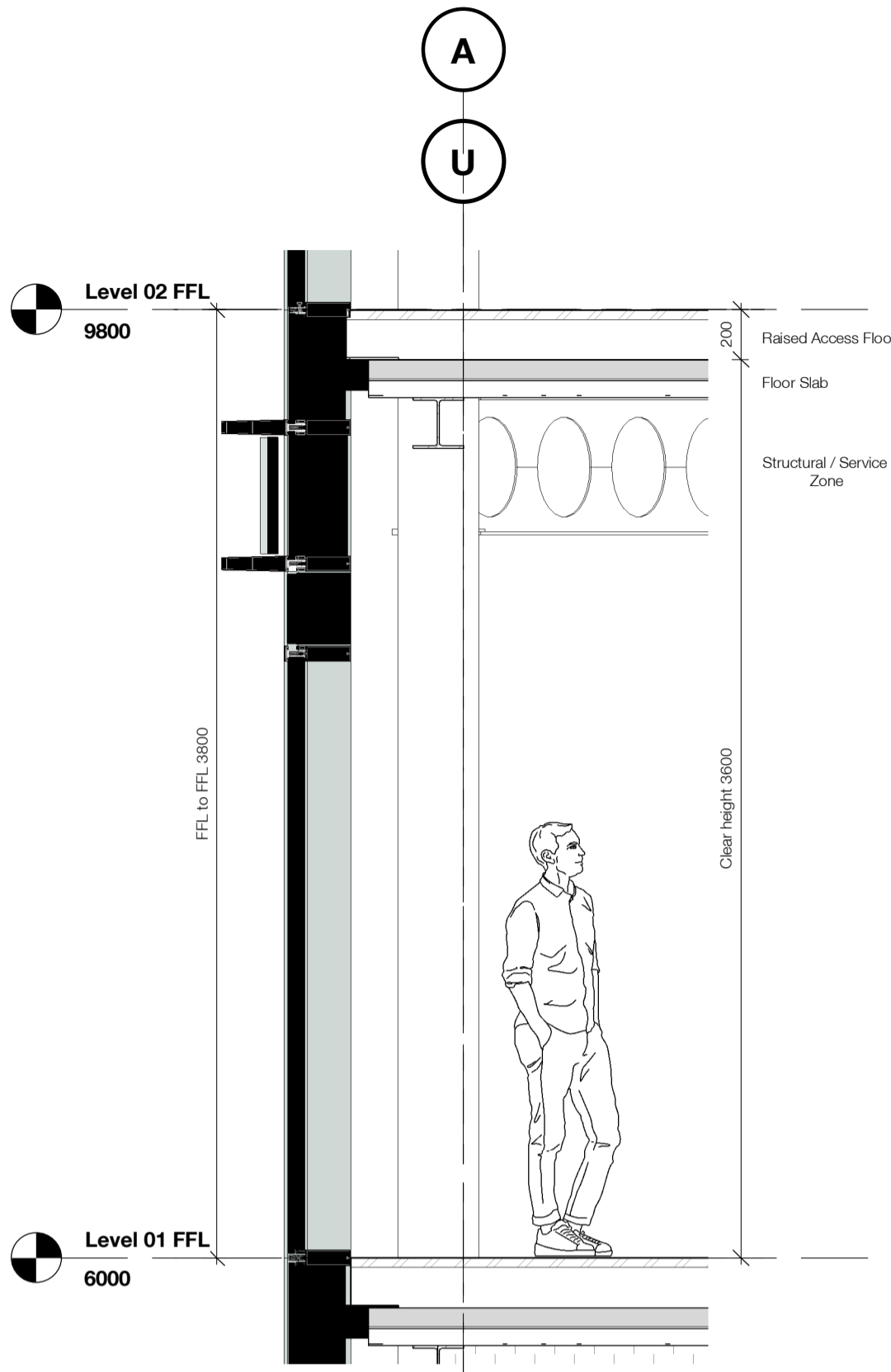
2 Section Call out 1:25
